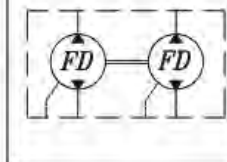
Flow Divider Symbol (with 2 sections)
