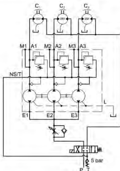
Flow divider application to control three motors
